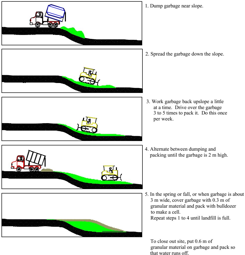
Figure 4-2 Depression Method
