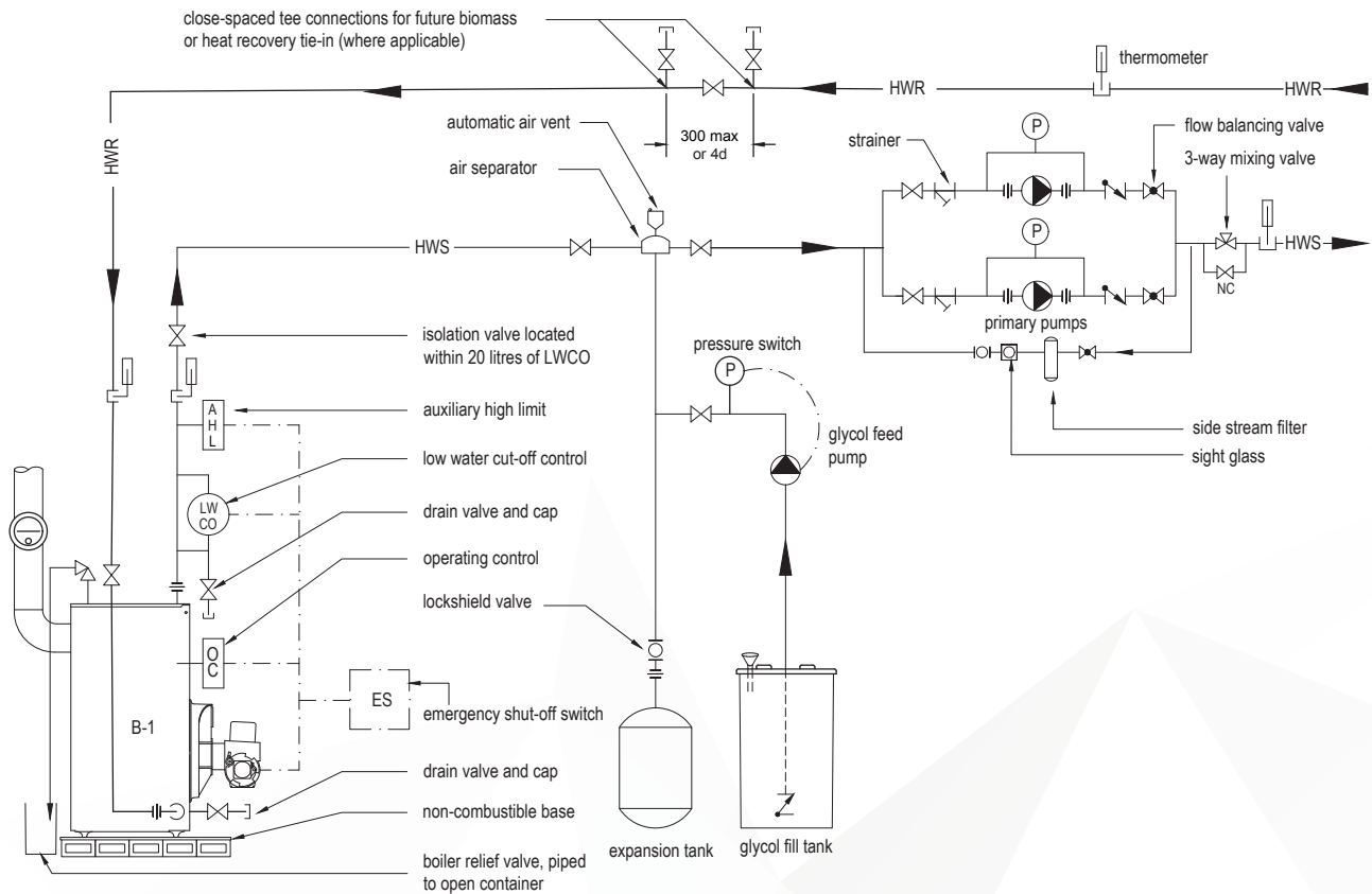
FIGURE 7-1: SINGLE BOILER DOUBLE PUMP
