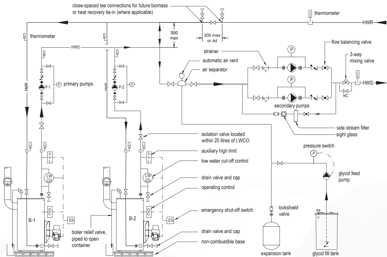
FIGURE 7-2: PRIMARY-SECONDARY BOILER SYSTEM
