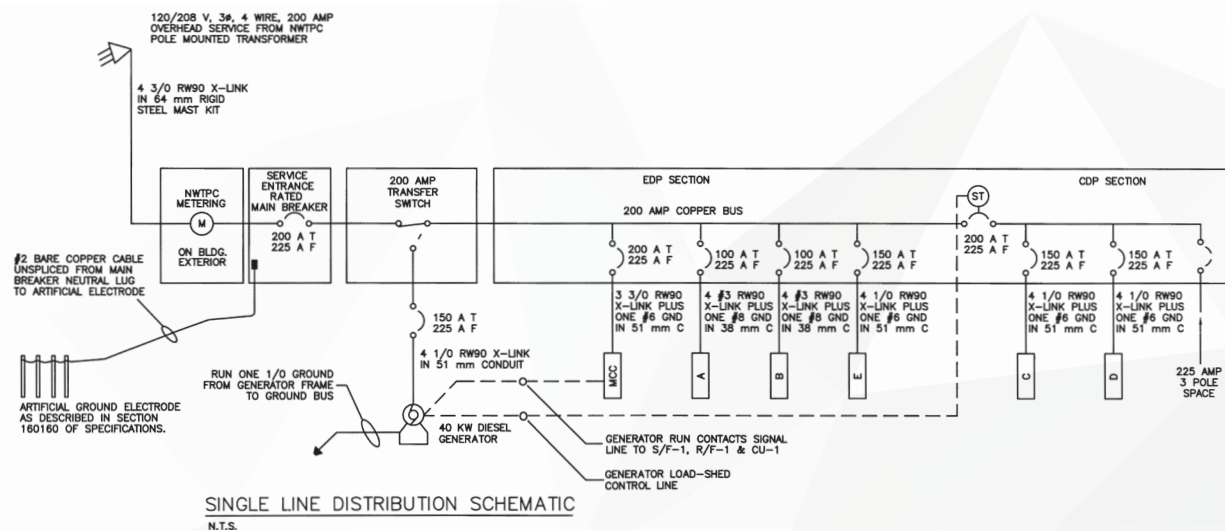
FIGURE 3-1: SAMPLE SINGLE LINE DIAGRAM
