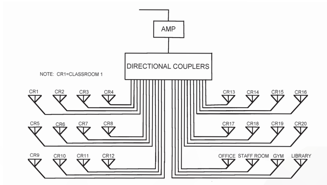
FIGURE 8-4: TYPICAL SCHOOL RFTV DISTRIBUTION SYSTEM
