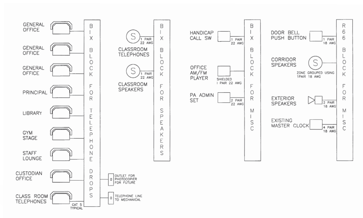
FIGURE 8-2: TYPICAL SCHEMATIC FOR ANALOG SCHOOL COMMUNICATIONS LAYOUT
