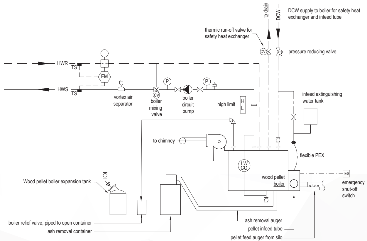
FIGURE 7- 4: WOOD PELLET BOILER WITH INTERNAL SAFETY HEAT EXCHANGER (HEX)
