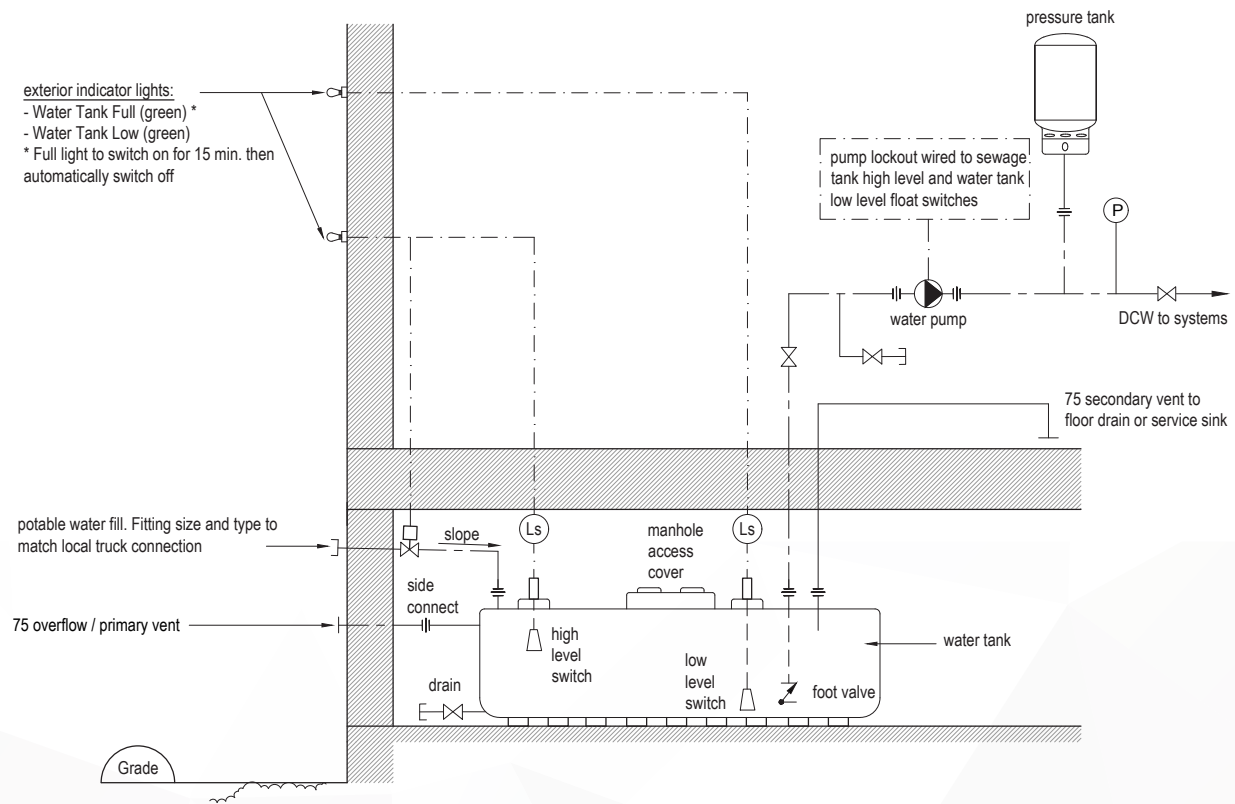
FIGURE 4-2: LARGE DOMESTIC WATER TANK (OVER 4200 LITRES)
