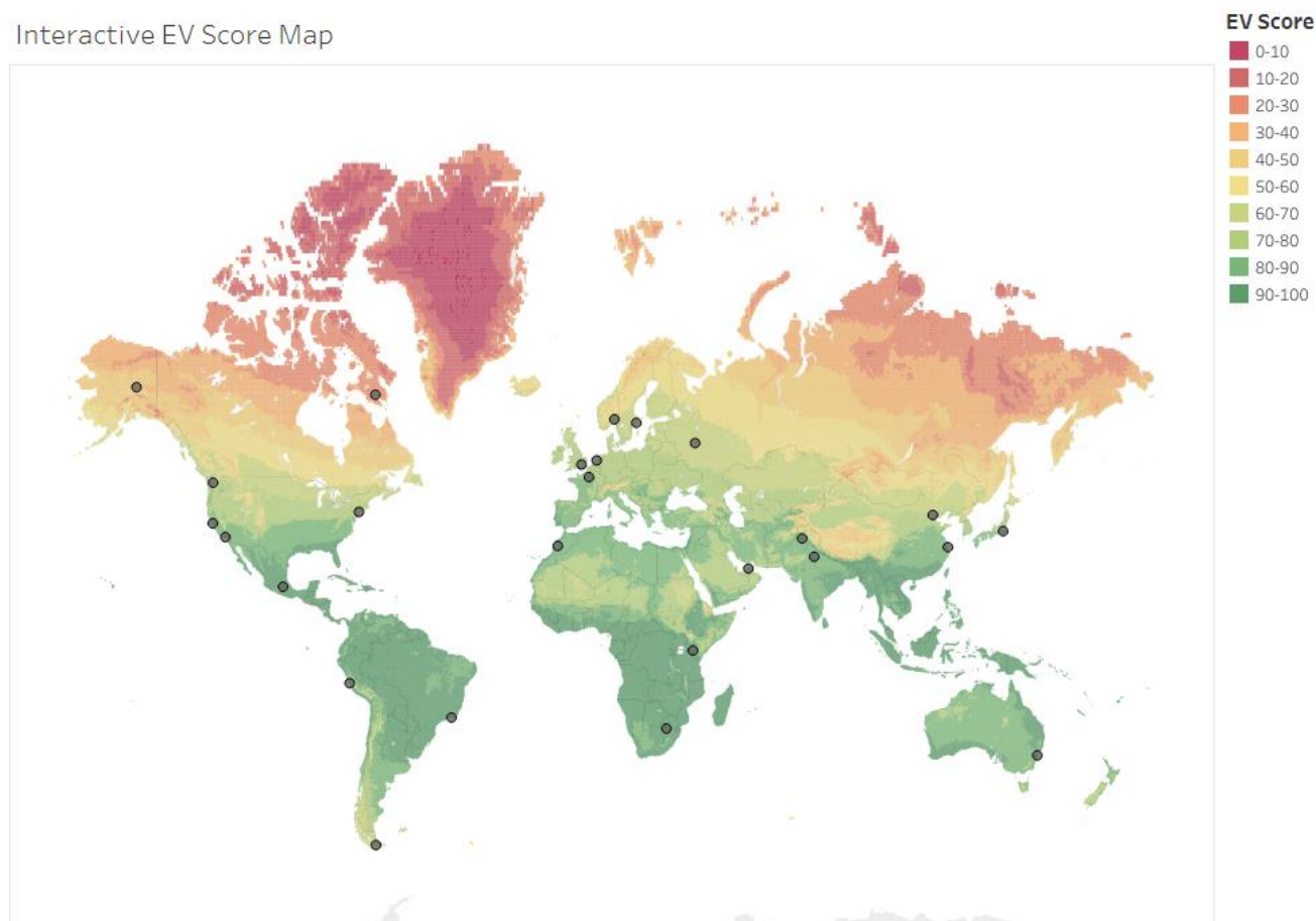
Figure 3: EV Score Map 7
