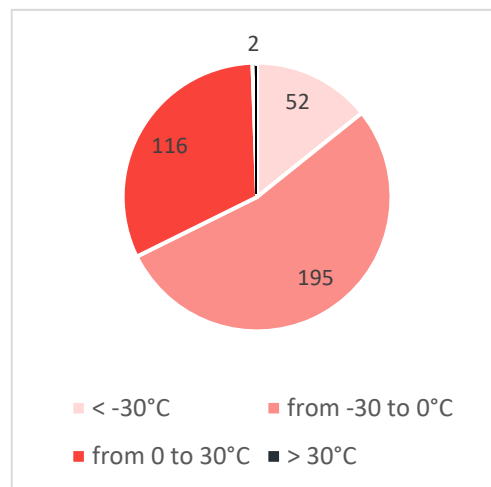
Figure 11 Historical average daily temperature for the NWT (1981-2010)
