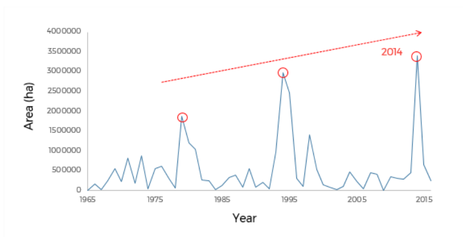
Figure 15 Forest area burned per year in the NWT between 1965 and 2016 (source: NWT Fire Management Division, 2016)
